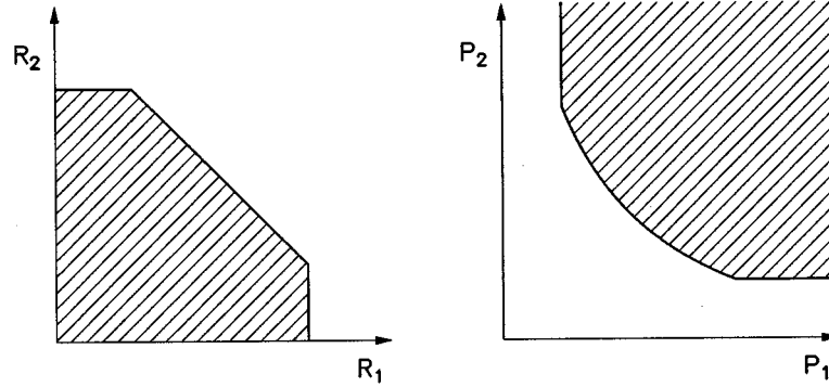
Fig. 8. Capacity and power regions for two users and |\rho_{12}|^2 = 0.85 .
