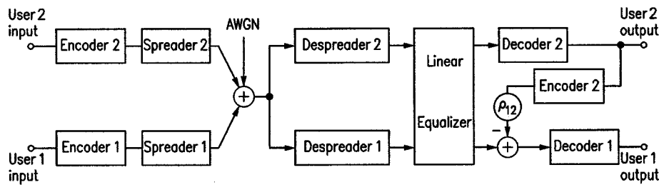
Fig. 4. Structure of decision-feedback decoding for two users.
