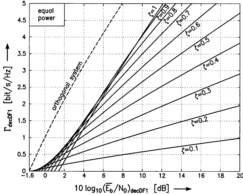
Fig. 5. Power-bandwidth-plane for the decorrelating decision-feedback receiver with load \zeta as parameter and equal powers for all users. For comparison the dashed line shows an orthogonal system.
