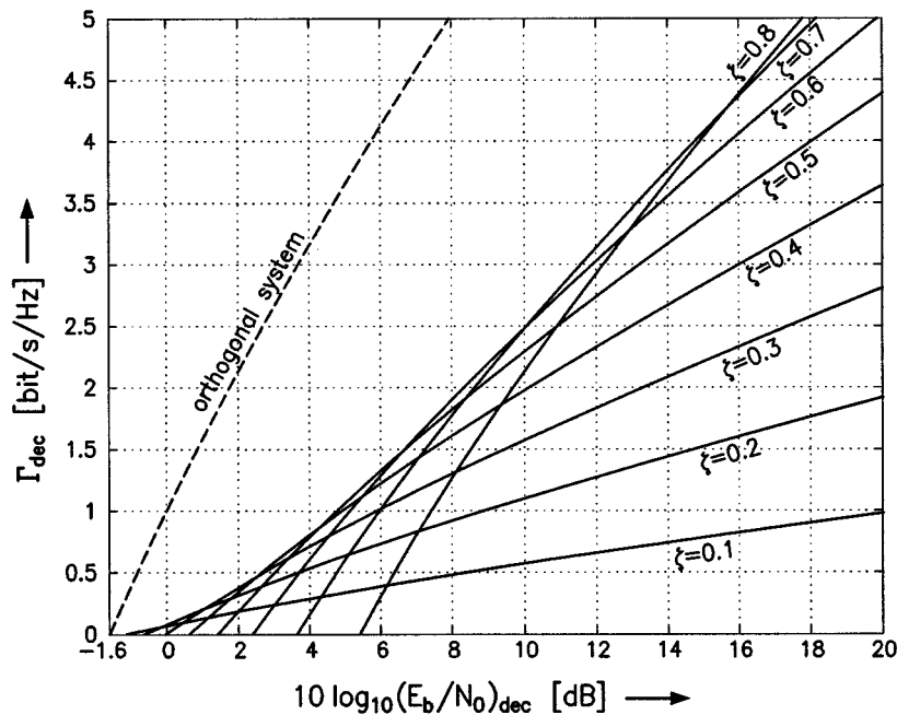
Fig. 2. Power-bandwidth-plane for the decorrelator with load \zeta as parameter. For comparison the dashed line shows an orthogonal system.
